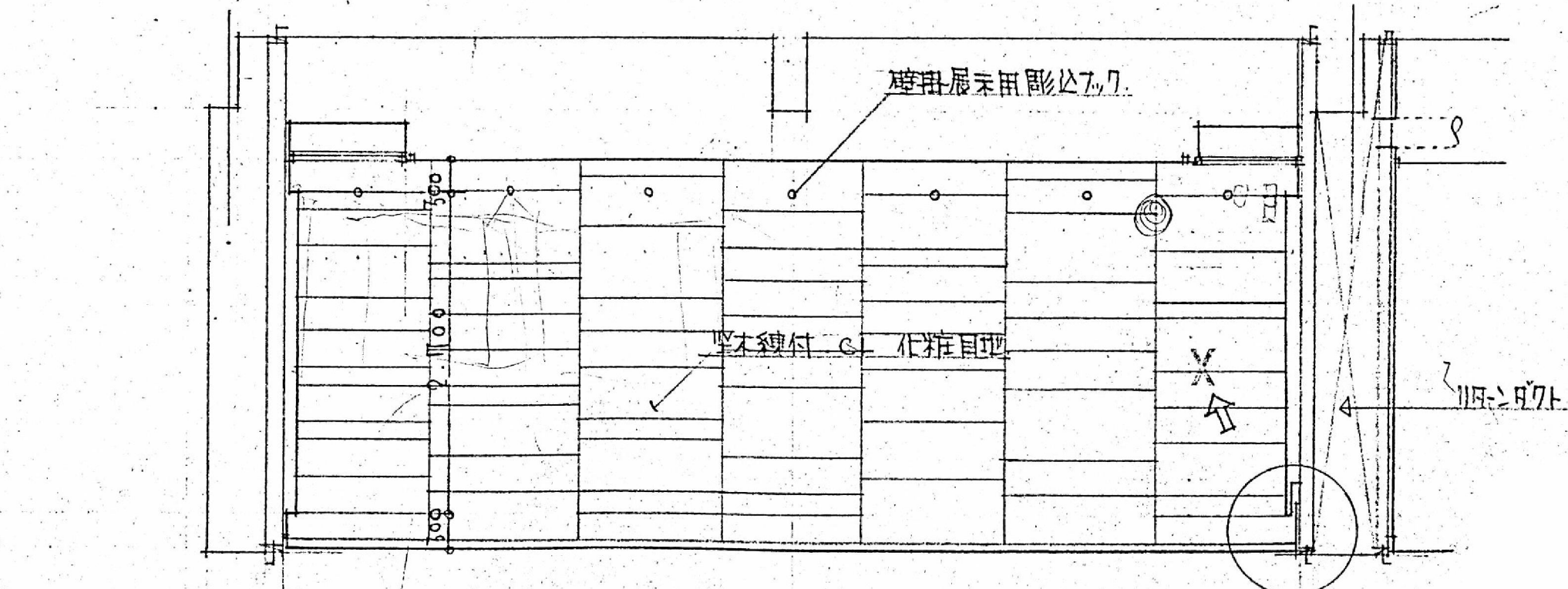
X部詳細 S: 1/20
