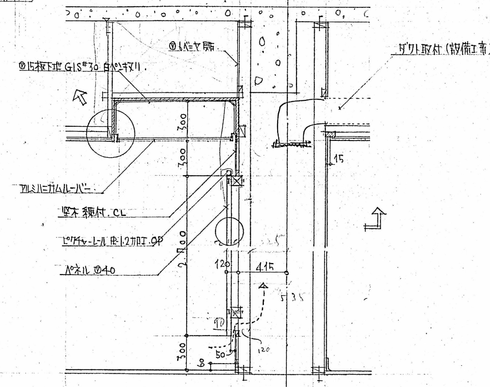
X部詳細 S: 1/20
